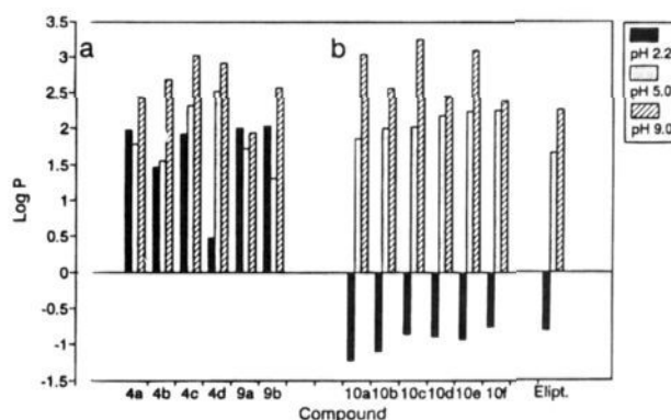
Figure 1. (a, b) Octanol-water partition coefficients of 5 H - and 6 H -indolo[2,3- b ]quinolines. Methanol containing 0.01% H 2 SO 4 was used as mobile phase (1.0 mL/min at 42 °C, 4.6 × 250 mm Supelcosil LC-18-DB column). All indolo[2,3- b ]quinolines had a retention time of 4.93 to 6.21; values of k = (v_r - v_0)/v_0 were 4a , 1.78; 4b , 1.86; 4c , 1.82; 4d , 1.84; 9a , 1.9; 10a , 2.19; 10b , 2.24; 10c , 2.12; 10d , 2.12; 10e , 2.22; 10f , 2.12; and for ellipticine, 2.40. v_0 for 4.6 × 250 mm Supelcosil LC-18-DB with precolumn filter was 2.77 mL.
